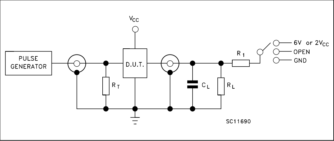
Figure 4. Test circuit
