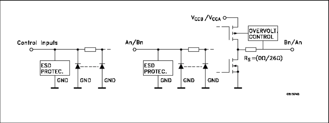
Figure 3. Input and output equivalent circuit
