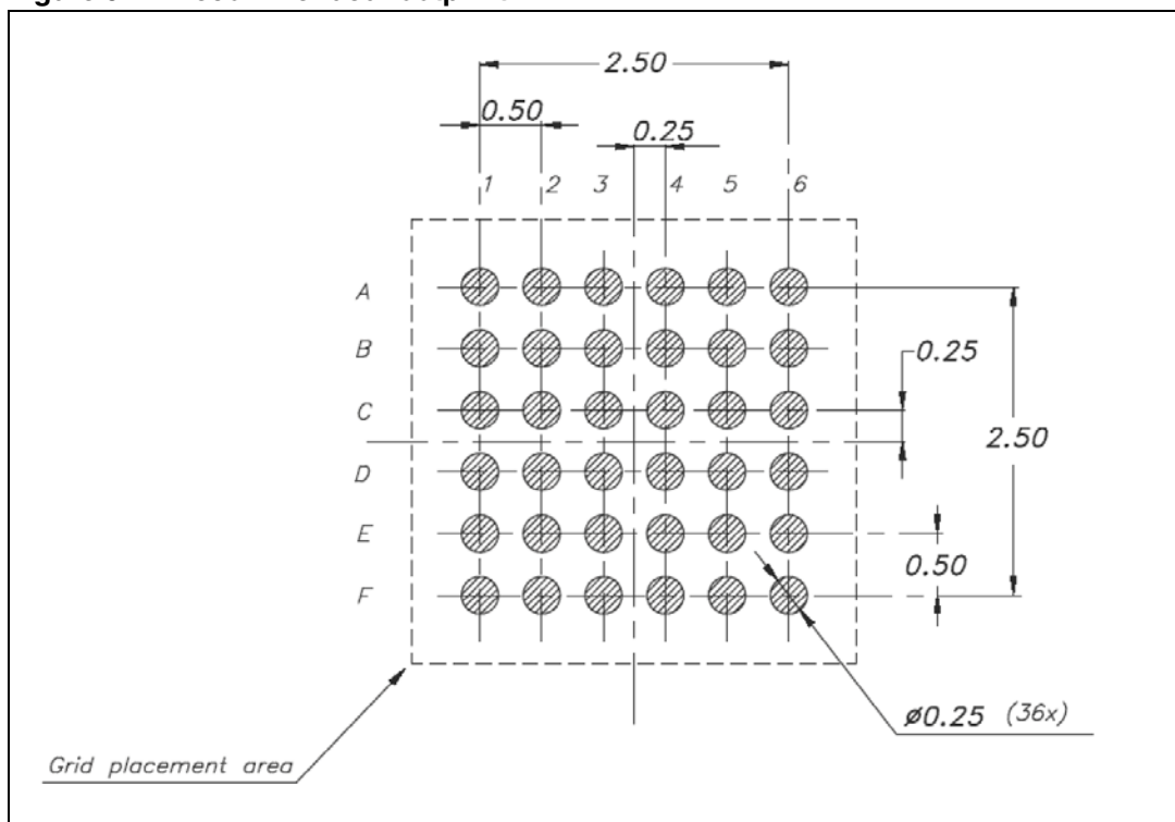
Figure 9. Recommended footprint
